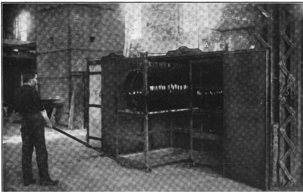
Tire japanning cabinet. Ovens with work charge in same on truck
